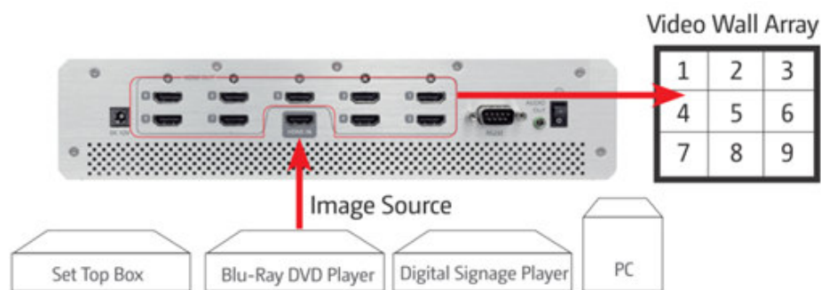
Figure 3-1: Cable Connection
