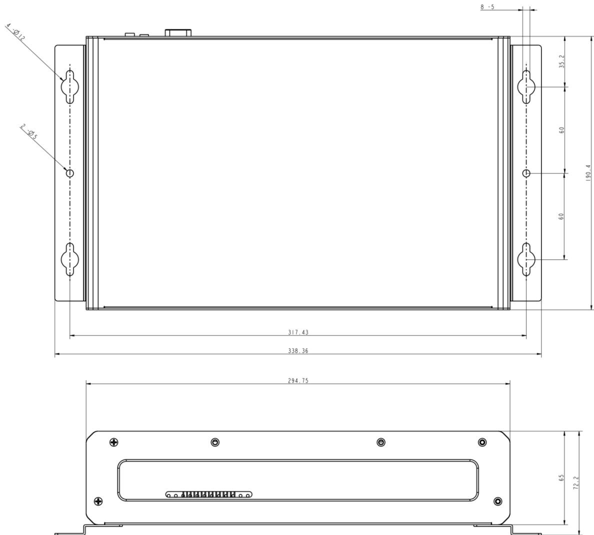
Figure 2-3: iVW-FH233 Dimensions
