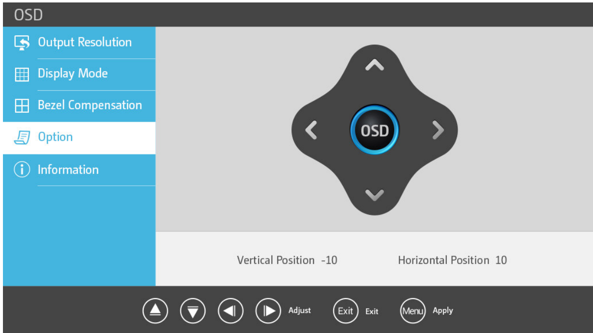
Figure 6-6: OSD Position Window
